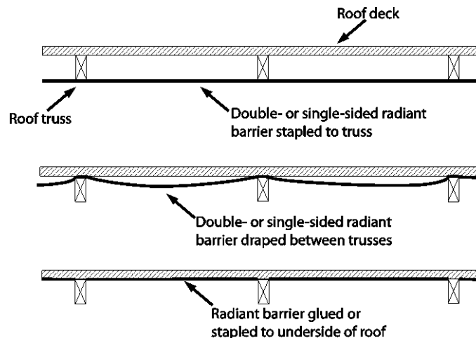
Figure 1 Attaching radiant barriers
